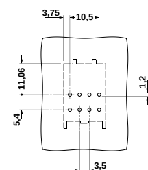
Drilling diagram VC-AMLV 8
