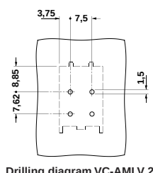
Drilling diagram VC-AMLV 2
