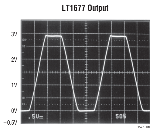
Figure 1. Voltage Follower with Input Exceeding the Supply Voltage ( V_S = 3\text{V} )
