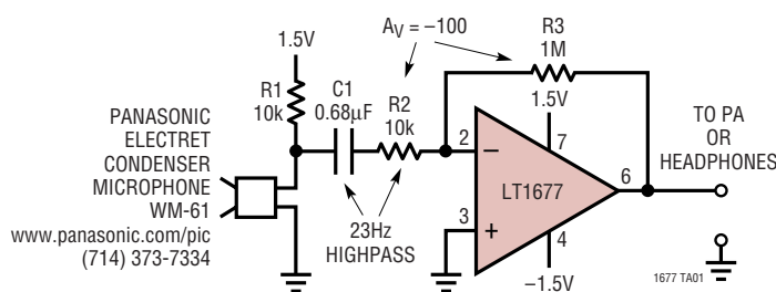
3V Electret Microphone Amplifier
