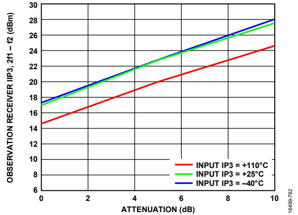
Figure 279. Observation Receiver IIP3, 2f_1 - f_2 vs. Attenuation, LO = 3600 MHz, Tone 1 = 3695 MHz, Tone 2 = 3696 MHz at -22 dBm Plus Attenuation
