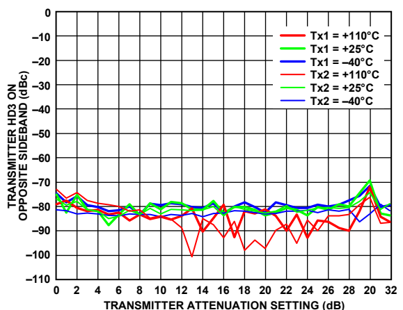
Figure 362. Transmitter HD3 on Opposite Sideband vs. Transmitter Attenuator Setting, LO = 5100 MHz, CW = -15 dBFS, Baseband Frequency = 10 MHz
