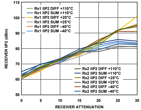
Figure 404. Receiver IIP2 vs. Receiver Attenuation, LO = 5800 MHz, Tones Placed at 5802 MHz and 5892 MHz, -21 dBm Plus Attenuation
