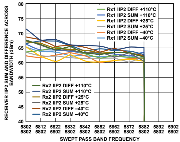
Figure 405. Receiver IIP2 Sum and Difference Across Bandwidth vs. Swept Pass Band Frequency, Receiver Attenuation = 0 dB, LO = 5800 MHz, Tone 1 = 5802 MHz, Tone 2 Swept, -21 dBm Each
