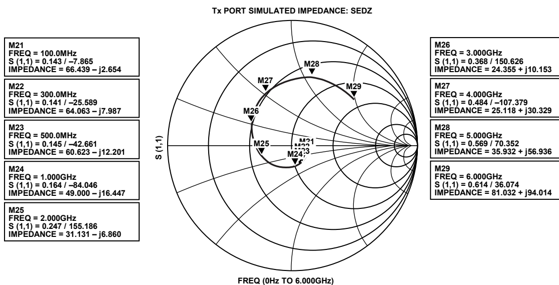
Figure 427. Transmitter Output Impedance Series Equivalent Differential Impedance (SEDZ)
