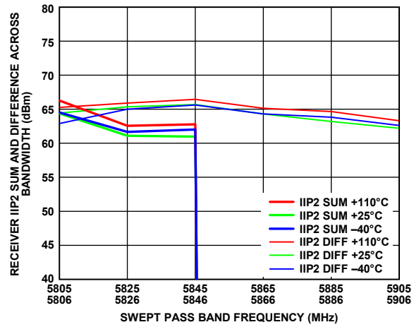
Figure 403. Receiver IIP2 Sum and Difference Across Bandwidth vs. Swept Pass Band Frequency, Receiver Attenuation = 0 dB, LO = 5800 MHz, Six Tone Pairs, -21 dBm Plus Attenuation Each
