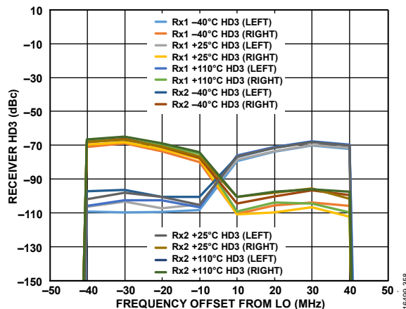
Figure 233. Receiver HD3 vs. Frequency Offset from LO, Tone Level = -15 dBm at Attenuation = 0, LO = 2850 MHz
