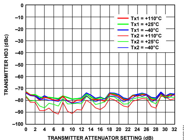
Figure 28. Transmitter HD3 vs. Transmitter Attenuator Setting, LO = 75 MHz, CW = -15 dBFS, Baseband Frequency = 10 MHz
