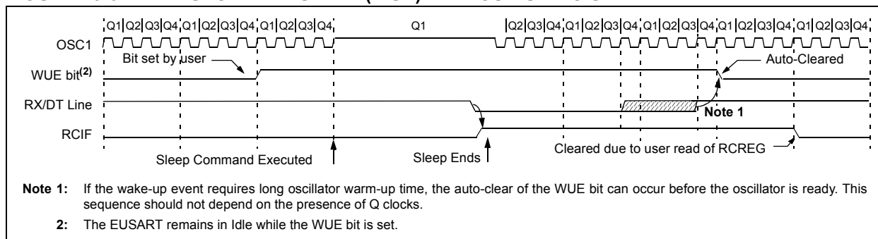
FIGURE 19-9: AUTO-WAKE-UP BIT (WUE) TIMINGS DURING SLEEP
