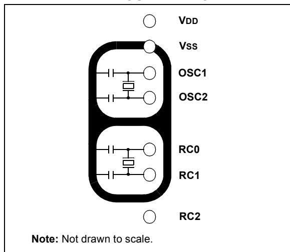
FIGURE 13-4: OSCILLATOR CIRCUIT WITH GROUNDED GUARD RING
