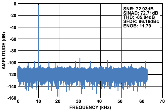
FIGURE 17. SINGLE-TONE FFT
