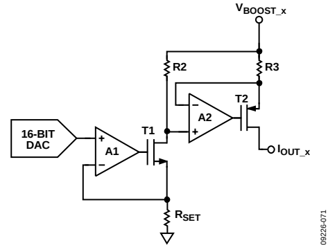
Figure 73. Voltage-to-Current Conversion Circuitry
