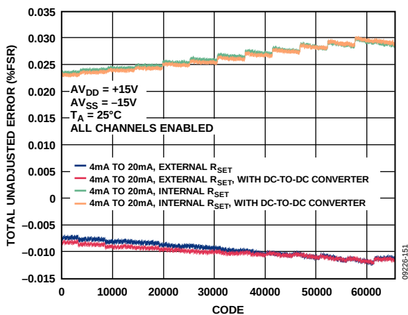
Figure 34. Total Unadjusted Error vs. Code
