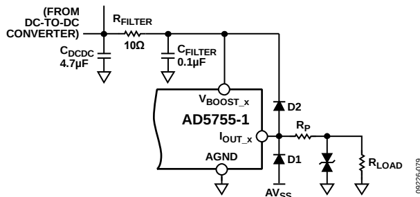
Figure 86. Output Transient Voltage Protection
