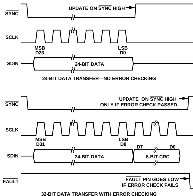
Figure 78. PEC Timing
