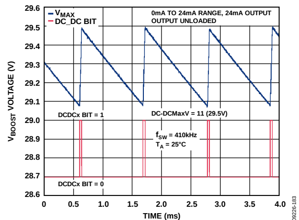
Figure 81. Operation on Reaching V_{\text{MAX}}
