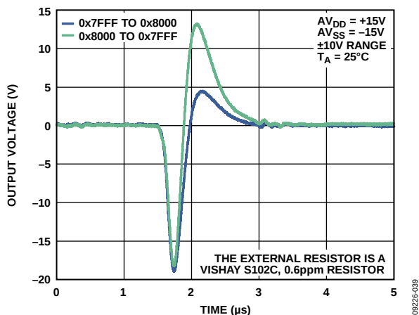
Figure 26. Digital-to-Analog Glitch
