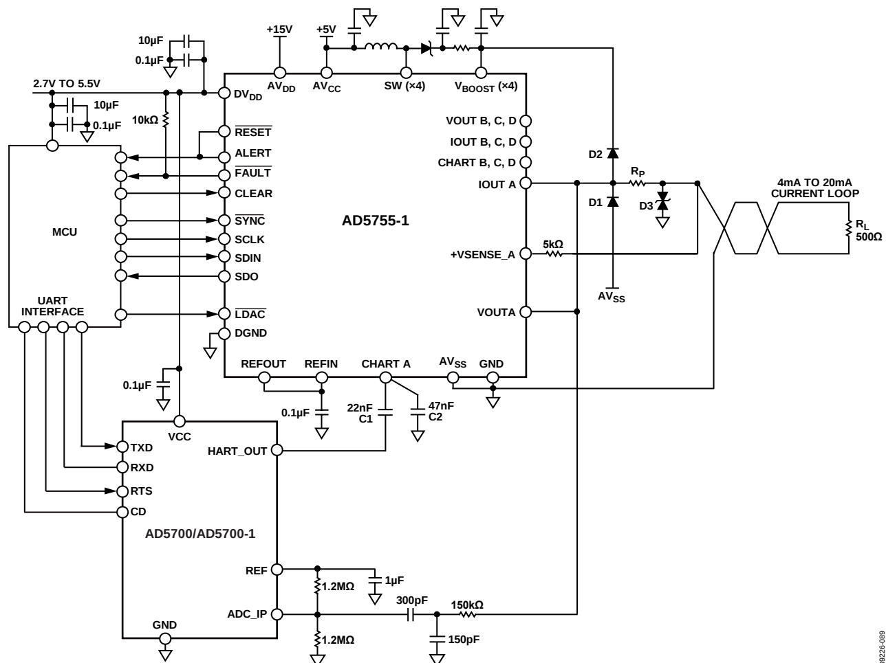
Figure 89. AD5755-1 in HART Configuration
