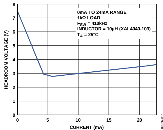
Figure 53. DC-to-DC Converter Headroom vs. Output Current (See Figure 80)
