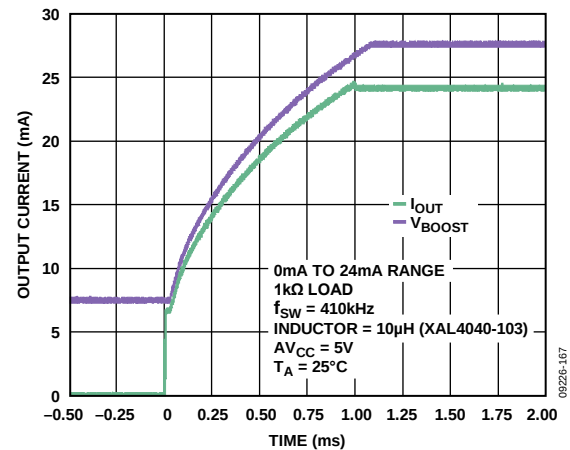
Figure 49. Output Current and V_{BOOST,X} Settling Time with DC-to-DC Converter (See Figure 80)
