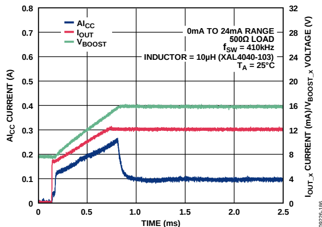
Figure 84. AI_{CC} Current vs. Time for 24 mA Step Through 500 \Omega Load with External 51 k \Omega Compensation Resistor
