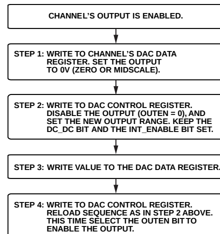
Figure 76. Steps for Changing the Output Range
