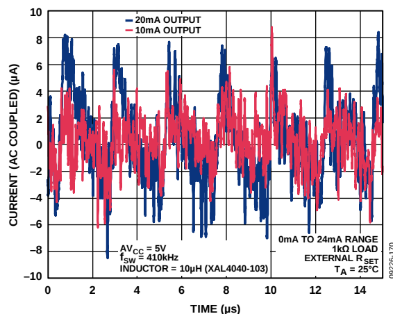
Figure 52. Output Current vs. Time with DC-to-DC Converter (See Figure 80)
