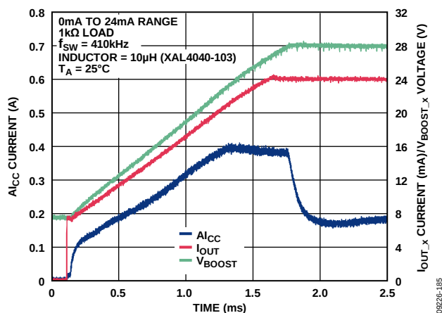
Figure 83. AI_{CC} Current vs. Time for 24 mA Step Through 1 k \Omega Load with External 51 k \Omega Compensation Resistor
