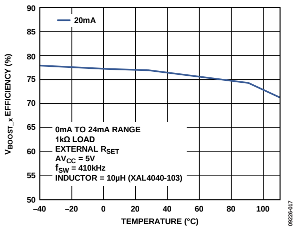
Figure 56. Efficiency at V_{BOOST\_X} vs. Temperature (See Figure 80)
