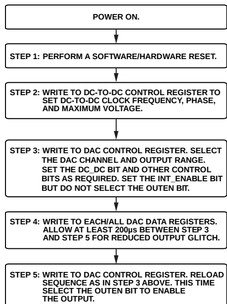
Figure 75. Programming Sequence for Enabling the Output Correctly
