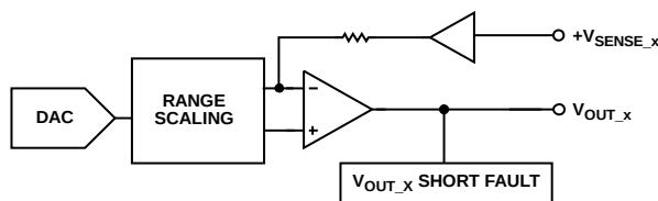
Figure 72. Voltage Output
