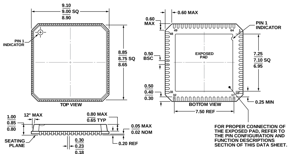
COMPLIANT TO JEDEC STANDARDS MO-220-VMMD-4 Figure 90. 64-Lead Lead Frame Chip Scale Package [LFCSP_VQ] 9 mm × 9 mm Body, Very Thin Quad (CP-64-3) Dimensions shown in millimeters
