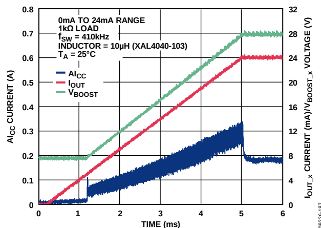
Figure 85. AI_{CC} Current vs. Time for 24 mA Step Through 1 k \Omega Load with Slew Rate Control
