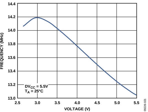
Figure 70. Internal Oscillator Frequency vs. DV_{CC} Supply Voltage
