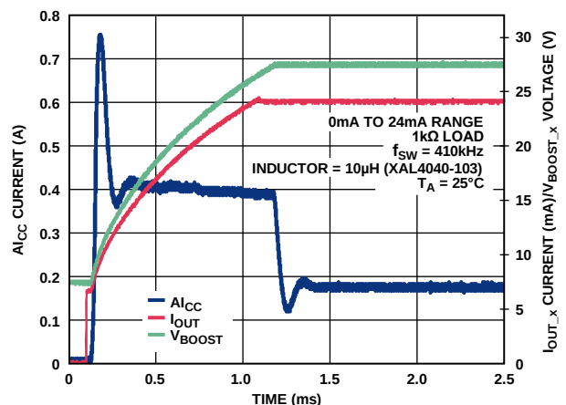
Figure 82. AI_{CC} Current vs. Time for 24 mA Step Through 1 k \Omega Load with Internal Compensation Resistor
