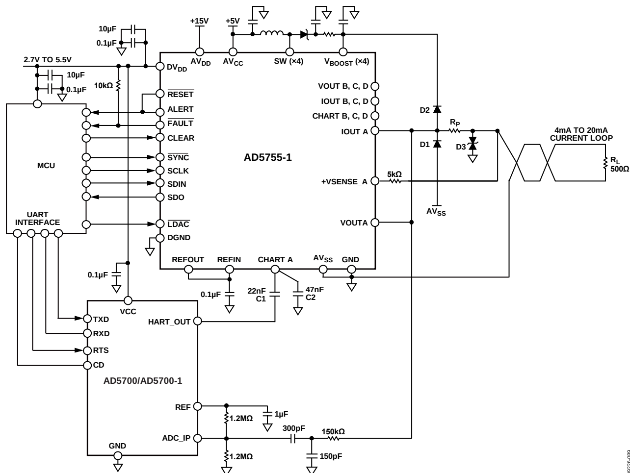
Figure 89. AD5755-1 in HART Configuration
