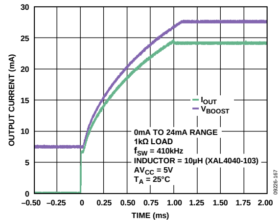
Figure 49. Output Current and V_{BOOST} Settling Time with DC-to-DC Converter (See Figure 80)
