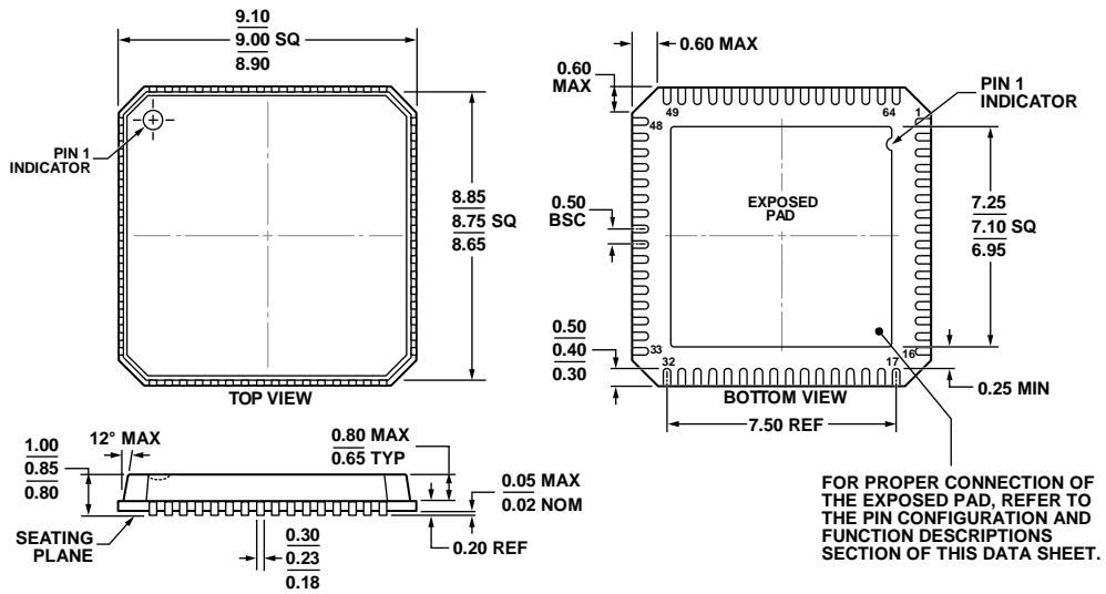
COMPLIANT TO JEDEC STANDARDS MO-220-VMM4-4 Figure 90. 64-Lead Lead Frame Chip Scale Package [LFCSP_VQ] 9 mm × 9 mm Body, Very Thin Quad (CP-64-3) Dimensions shown in millimeters
