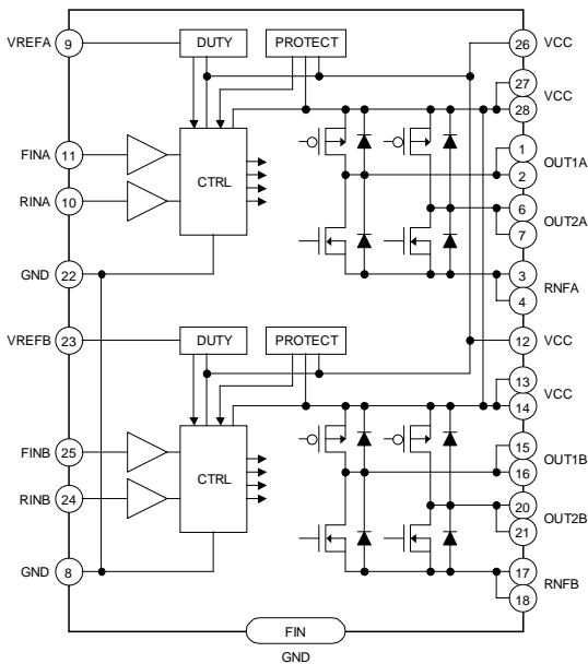
Fig.11 BD6237FM
