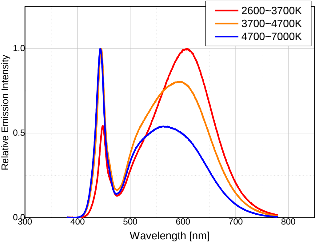
Fig 1. Color Spectrum, I_F=20\text{mA} , T_j=25^\circ\text{C} , RH30%
