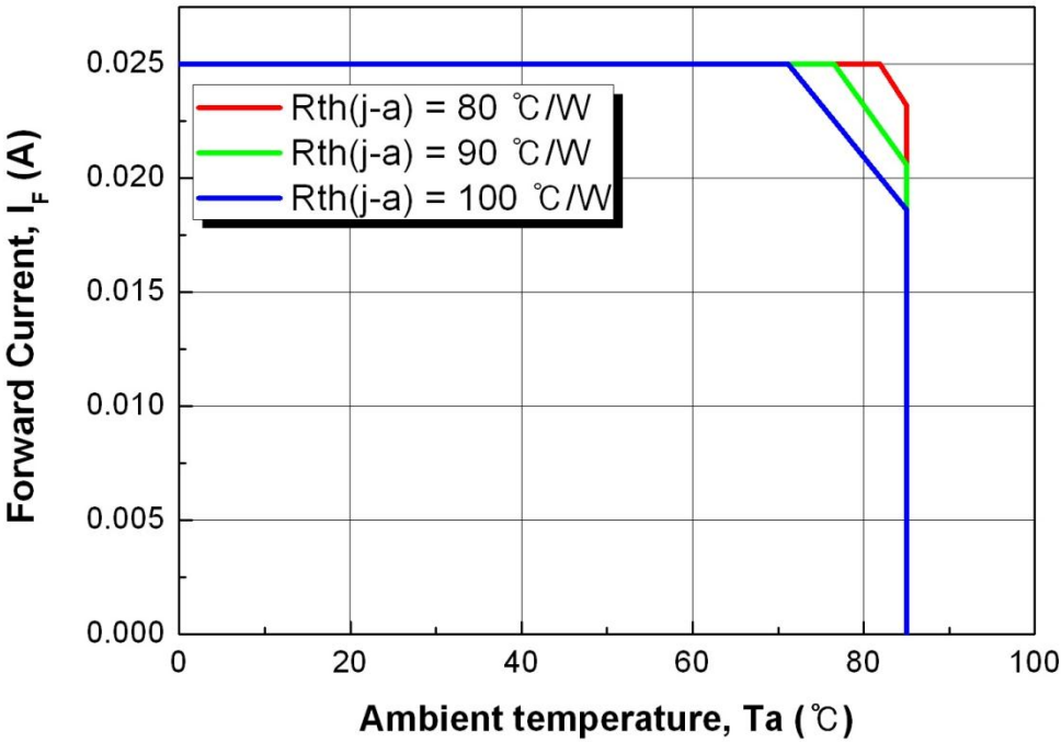
Fig 9. Maximum Forward Current vs. Ambient Temperature, T_j(max.) = 125^{\circ}C , I_F=25mA
