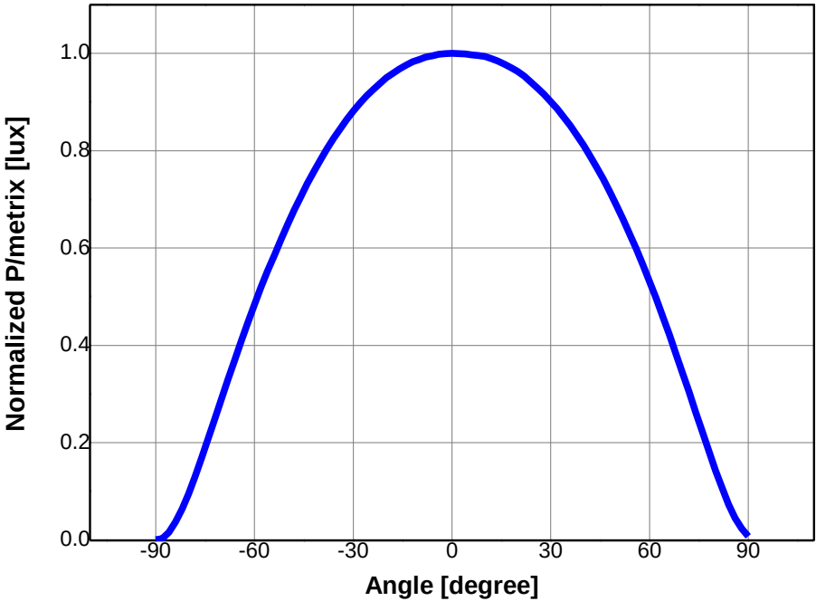
Fig 2. Radiant pattern, I_F = 20\text{mA}
