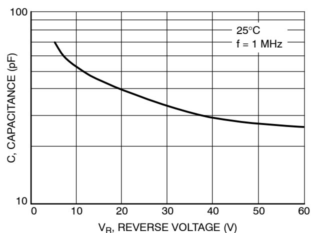
Figure 4. Typical Capacitance
