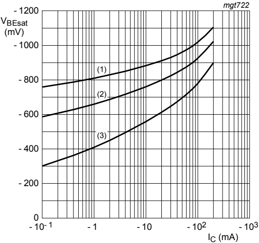
Figure 10. BC857C: Base-emitter voltage as a function of collector current; typical values
