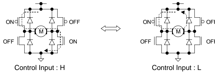
Figure 34. PWM Control Mode A Operation (Output Stage)
