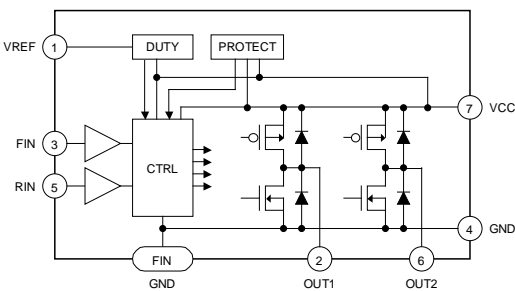
Figure 3. BD6222HFP
