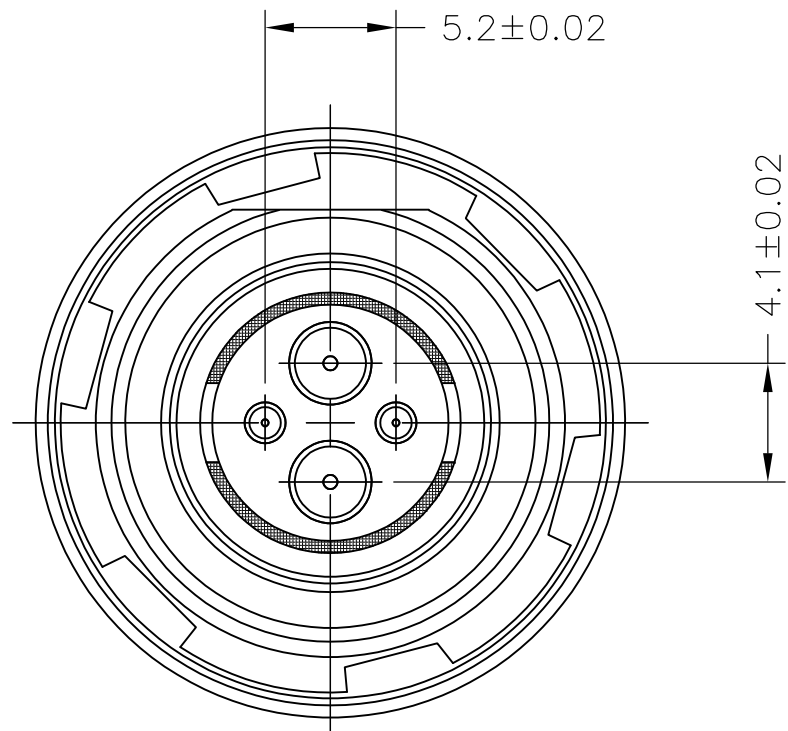
DOUBLE POLARIZATION
