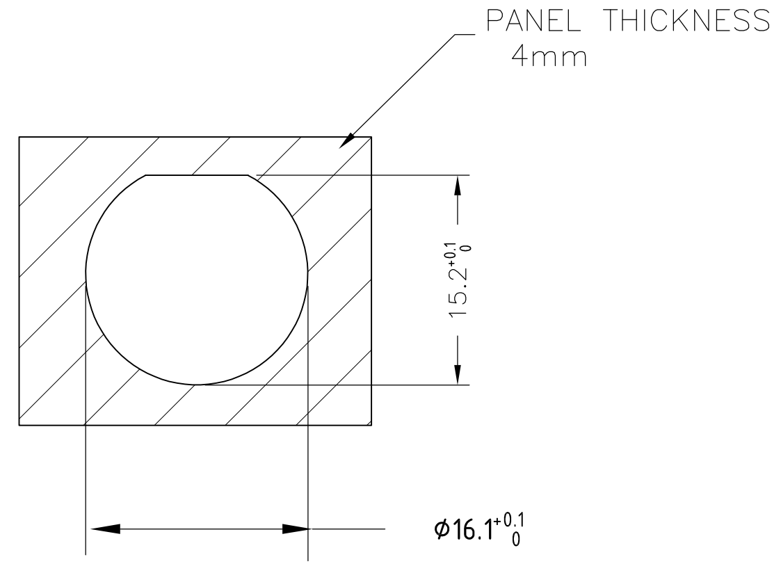
PANEL CUTOUT
