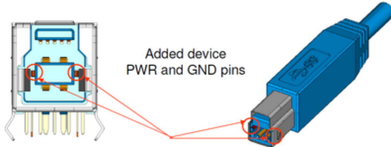
Figure 8 : USB 3.0 Powered-B Connector USB 3.0 includes a variant of the Standard-B connectors which has two additional conductors to provide power to USB adapters. Image courtesy of USB Implementers Forum
