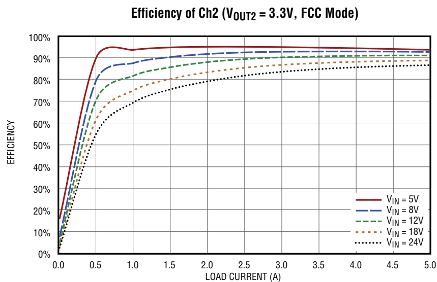
Figure 3. Measured Efficiency on Channel 2 V_{OUT2} = 3.3V , f_{SW} = 500kHz , CCM, Channel 1, 3 Disabled
