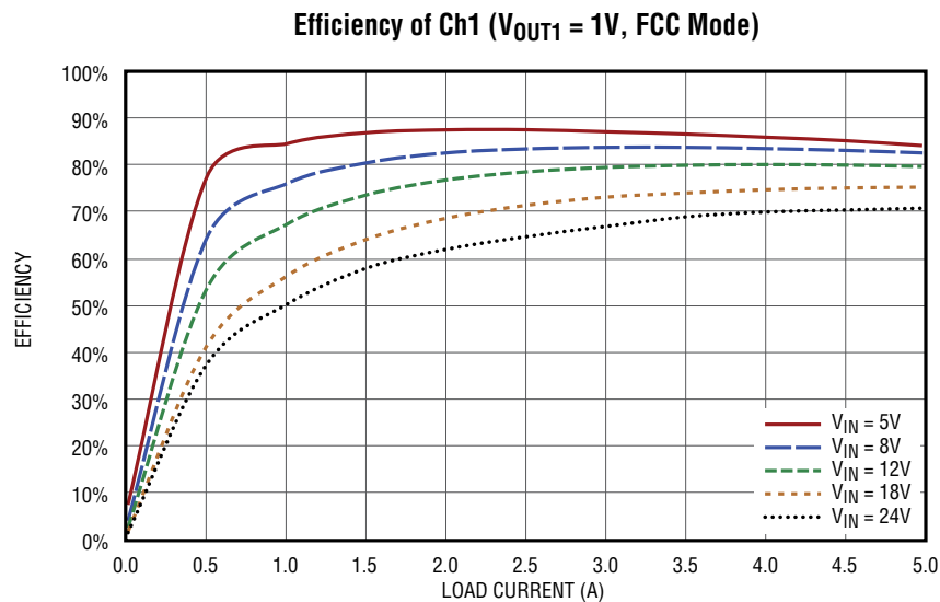
Figure 2. Measured Efficiency on Channel 1 V_{OUT1} = 1.0V , f_{SW} = 500kHz , CCM, Channel 2, 3 Disabled
