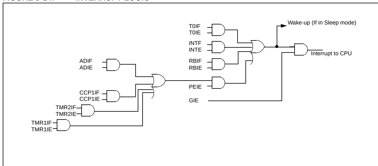
FIGURE 9-14: INTERRUPT LOGIC
