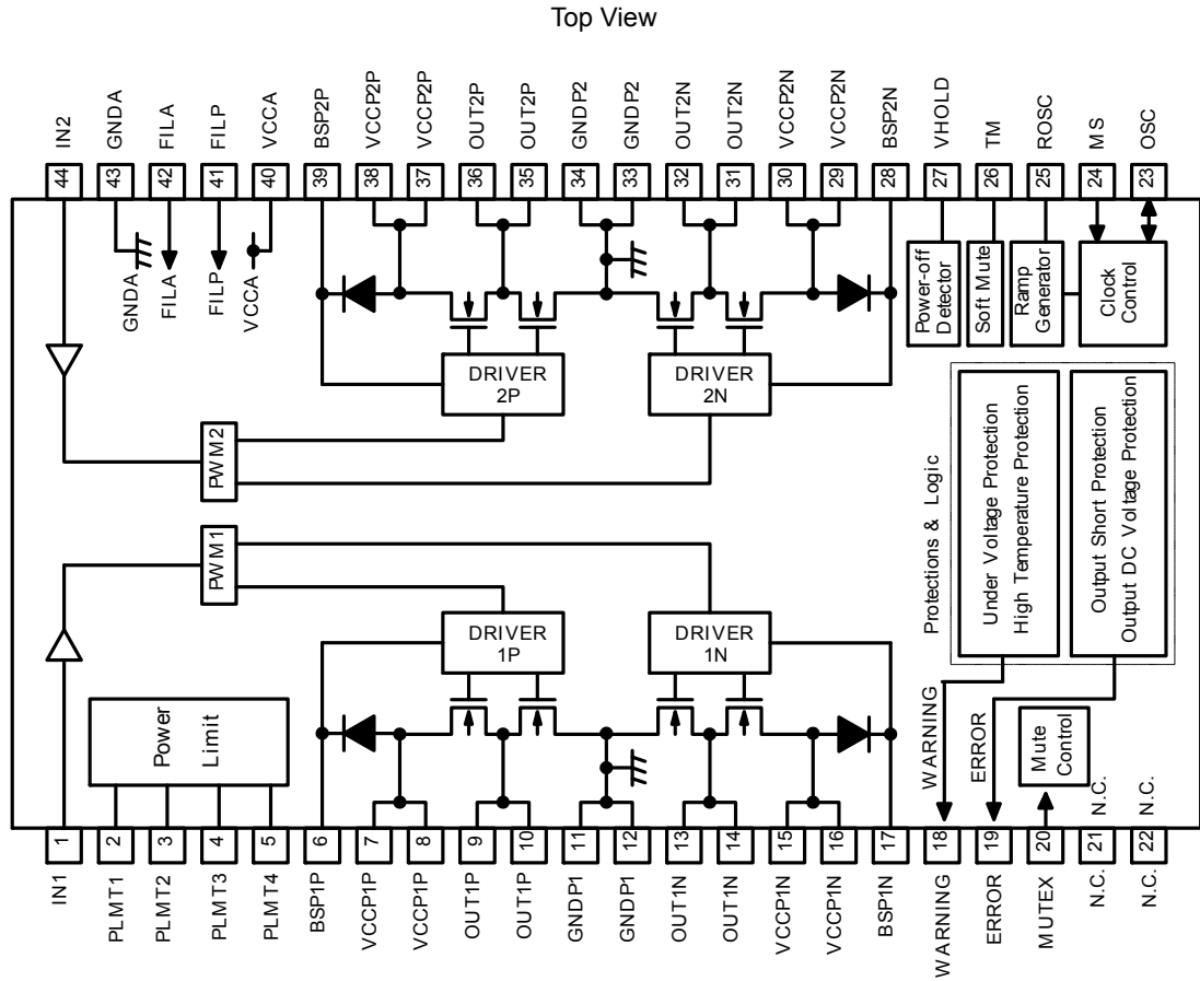
Fig. 28 Pin Assignment Diagram
