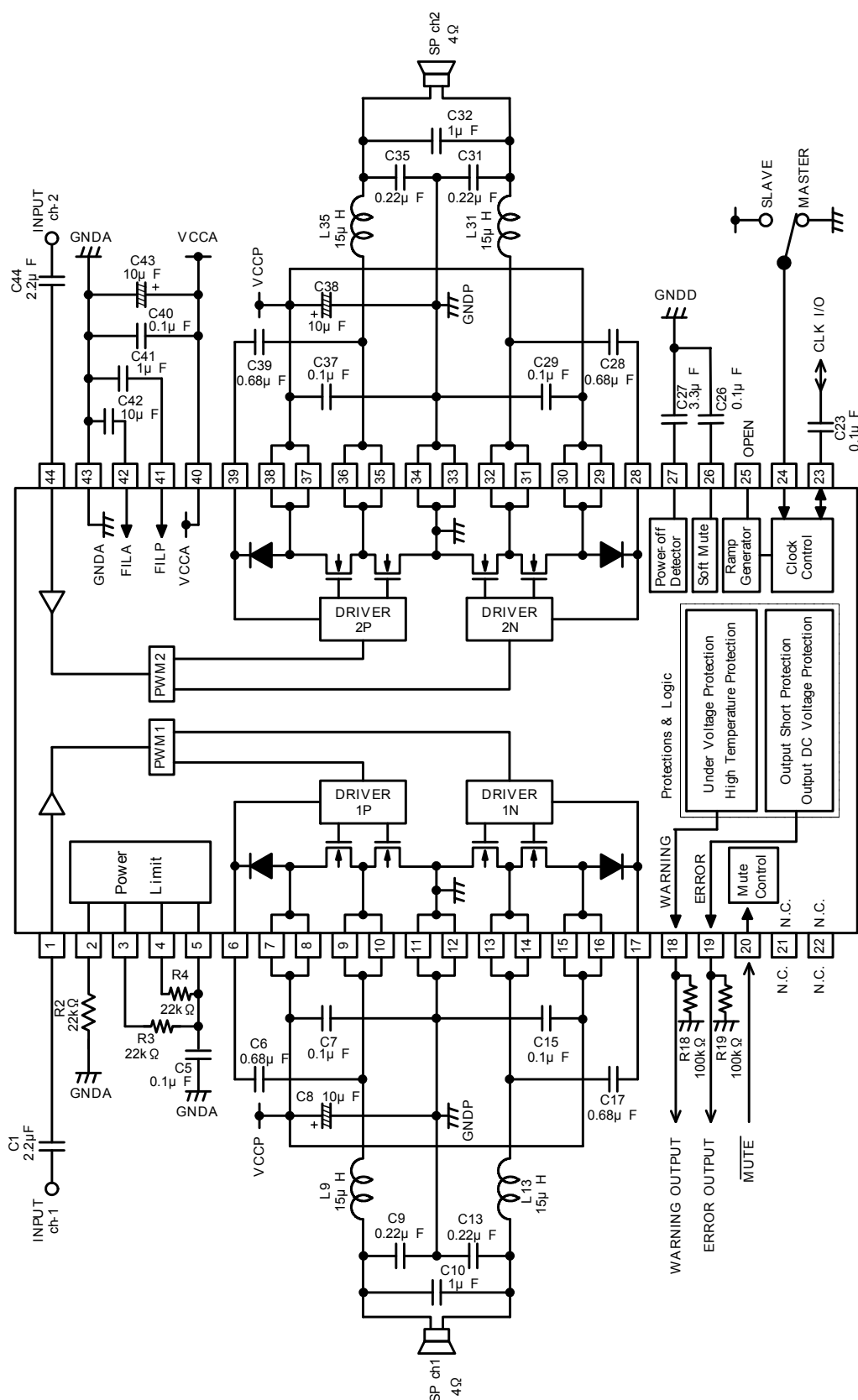
Fig. 30 Circuit diagram under stereo operation with 4- \Omega load
