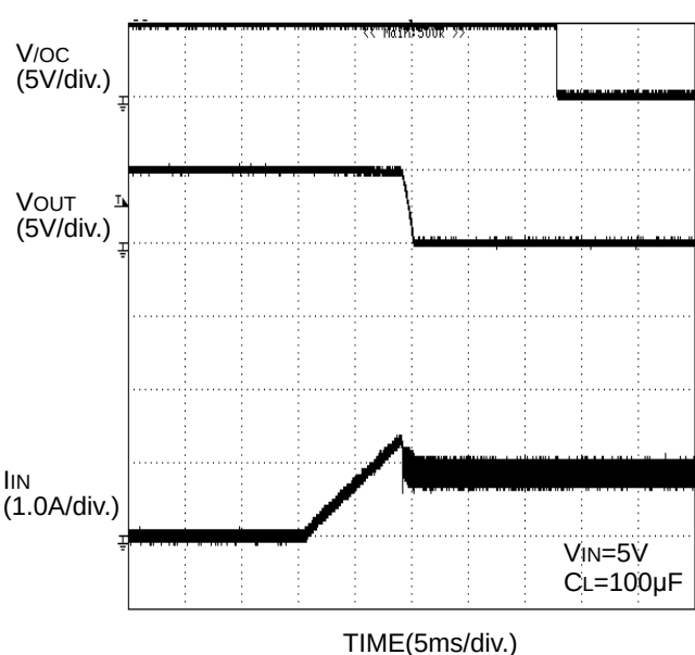
Figure 35. Over-Current Response Ramped Load
