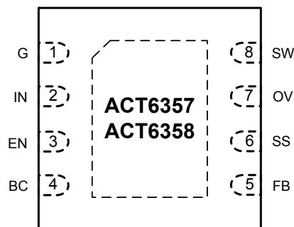
TDFN33-8
