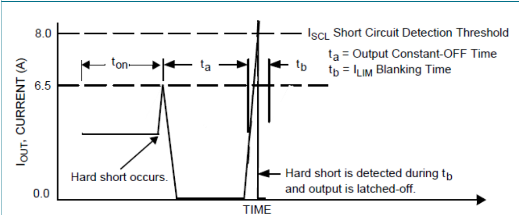
Figure 11. Example short-circuit detection detail on low-side MOSFET
