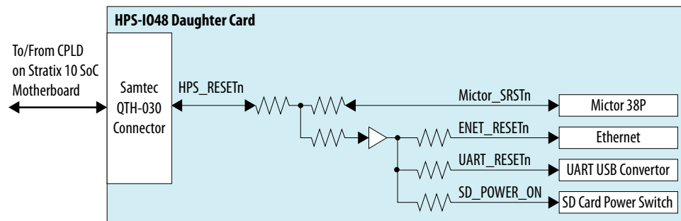
Figure 17. Reset Diagram
