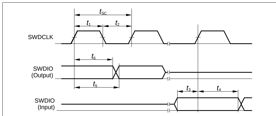
Figure 29 SWD Timing
