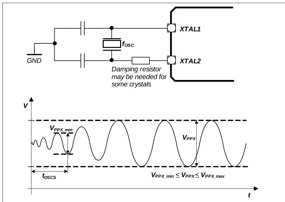
Figure 20 Oscillator in Crystal Mode
