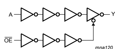
Figure 3. Logic diagram
