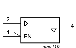
Figure 2. IEC logic symbol
