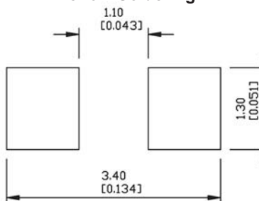
Recommended Soldering Pattern For Reflow Soldering
