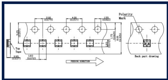
1210 BI-COLOR PACKAGE
