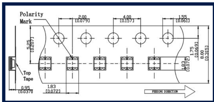
1210 TRI-COLOR PACKAGE
