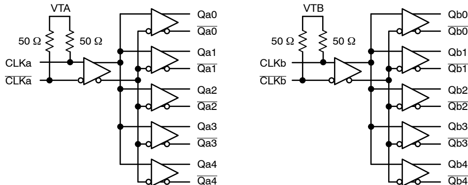
Figure 2. Logic Diagram
