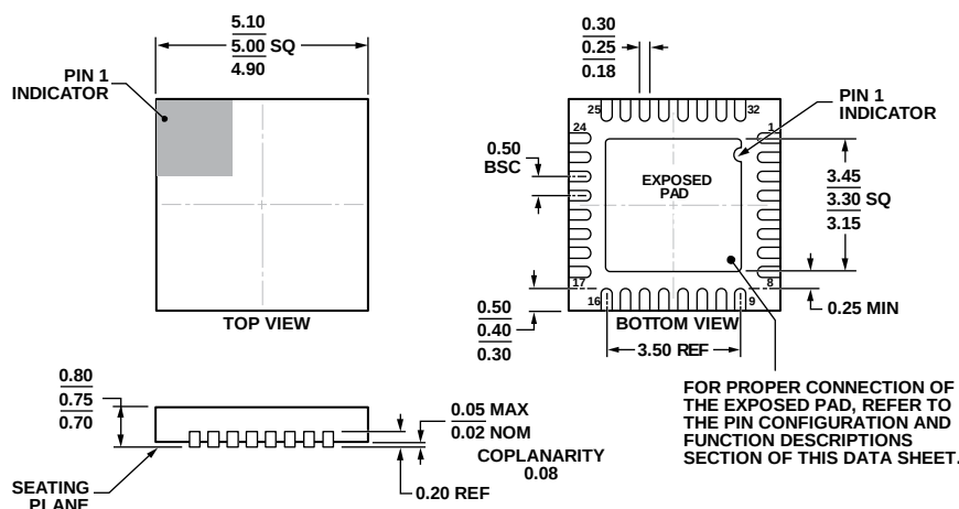
Figure 89. 32-Lead Lead Frame Chip Scale Package [LFCSP_WQ]
