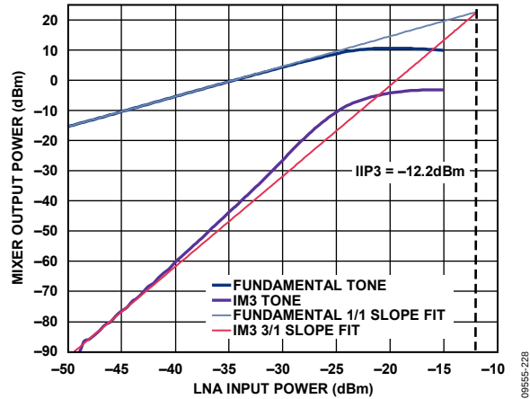
Figure 17. LNA/Mixer IIP3, V_{DD} = 3.0\text{ V} , Temperature = 25^\circ\text{C} , RF Frequency = 915 MHz, LNA Gain = High, Mixer Gain = High, Source 1 Frequency = (915 + 0.4)\text{ MHz} , Source 2 Frequency = (915 + 0.7)\text{ MHz}
