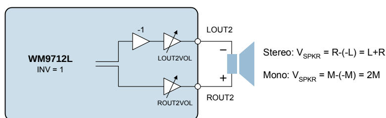
Figure 27 Speaker Output Connection (INV = 1)
