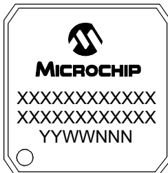
121-BGA (10x10x1.1 mm)
