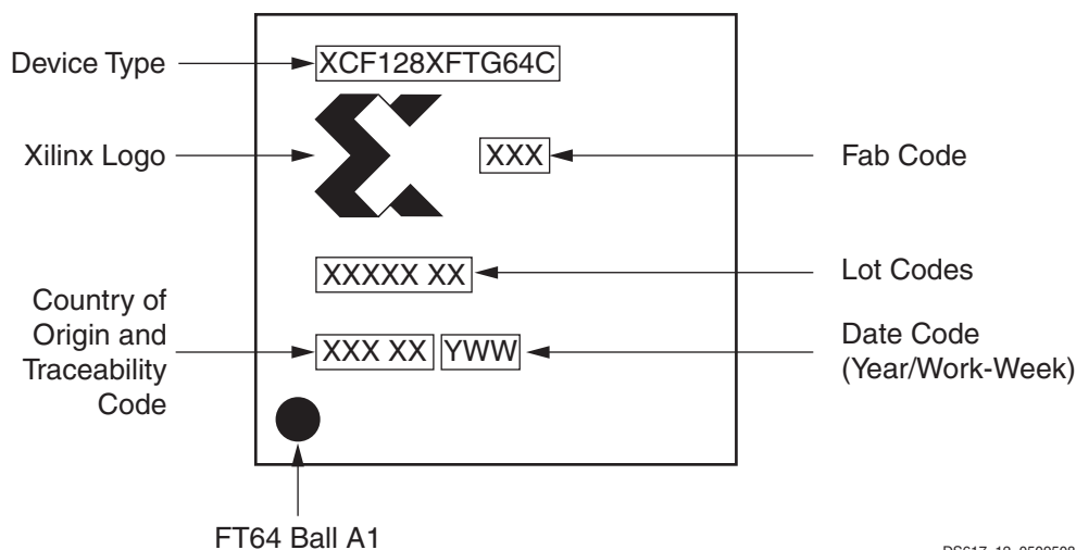
Figure 36: Marking Information
