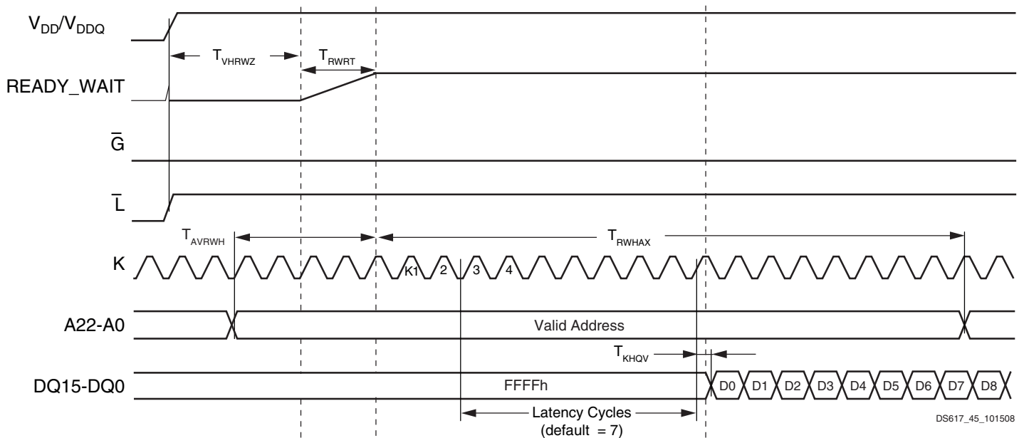
Figure 11: Power-Up
