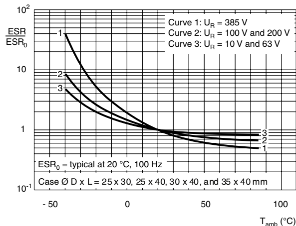
Fig.13 Typical multiplier of ESR as a function of ambient temperature.
