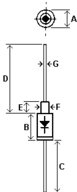
DO-13 (DO-202AA)
