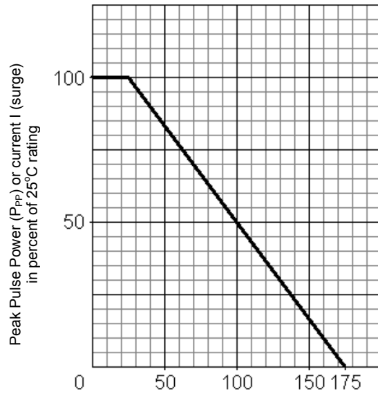
TA Ambient Temperature °C FIG. 4 Derating Curve
