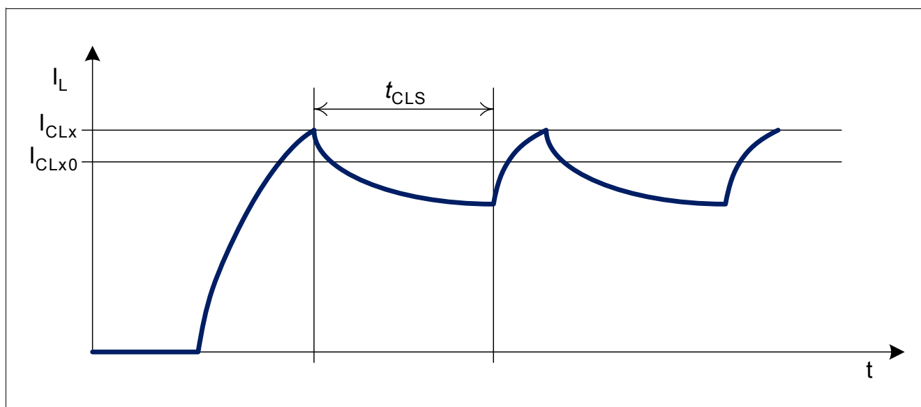
Figure 9 Timing diagram current limitation (inductive load)
