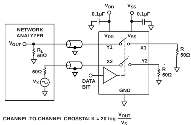
Figure 32. Channel-to-Channel Crosstalk
