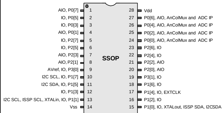
Figure 5. CY8C24533 PSoC Device
