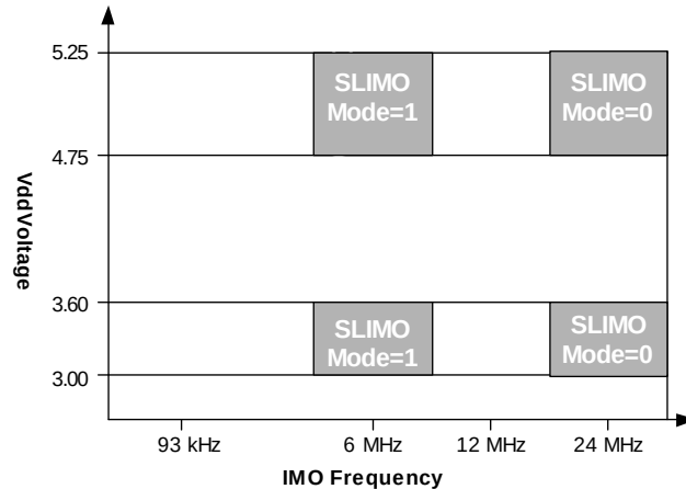
Figure 7. IMO Frequency Trim Options
