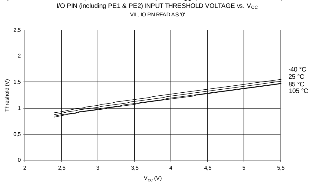
Figure 24-20. I/O Pin Input Threshold Voltage vs. V_{CC} ( V_{IL} , I/O Pin Read As '0')
