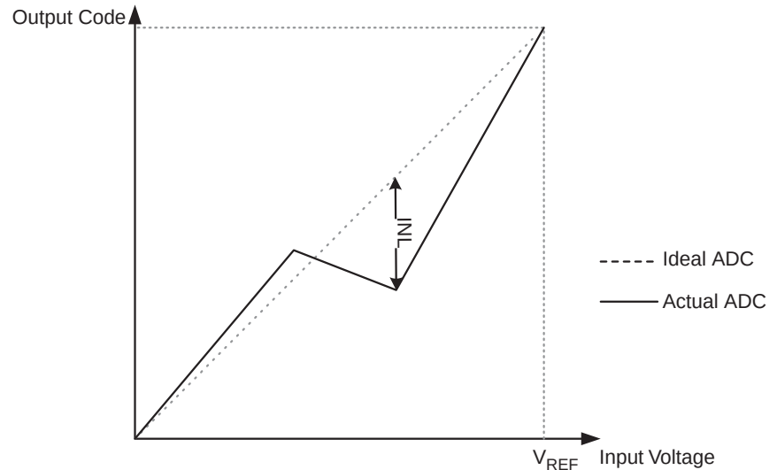
Figure 19-12. Integral Non-linearity (INL)
