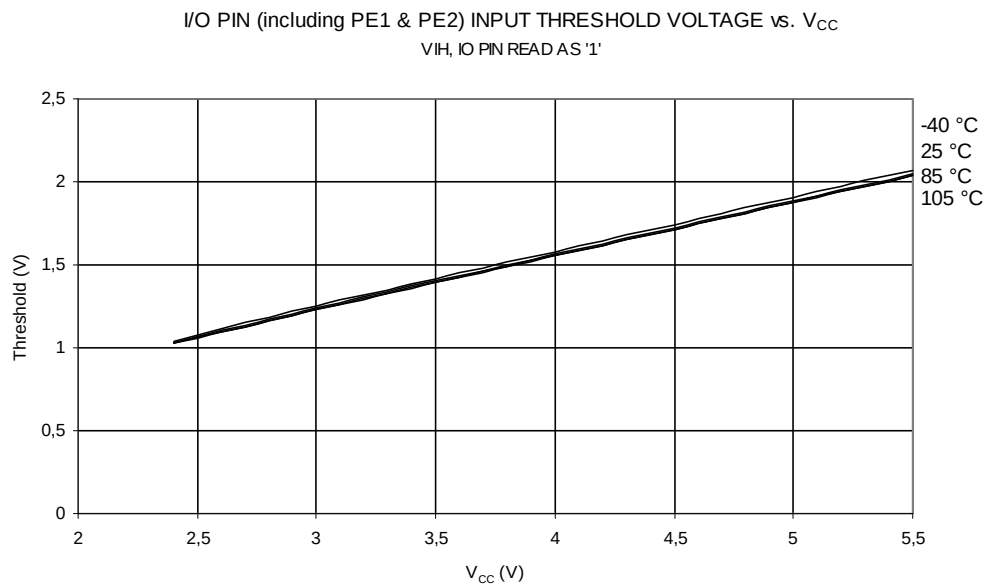
Figure 24-19. I/O Pin Input Threshold Voltage vs. V_{CC} ( V_{IH} , I/O Pin Read As '1')
