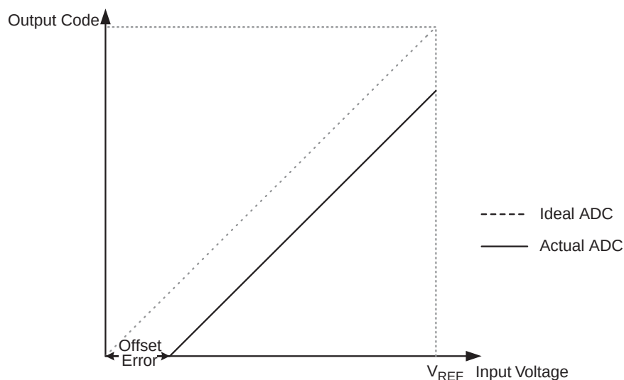
Figure 19-10. Offset Error
