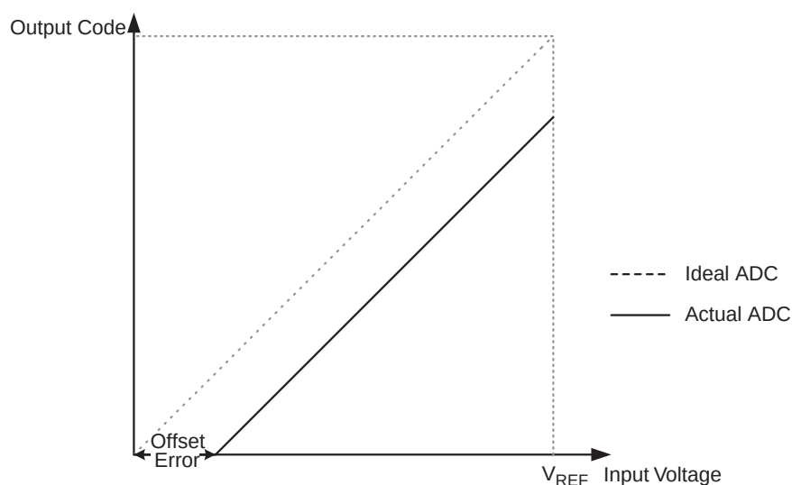
Figure 19-10. Offset Error
