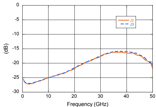
Output Return Loss @ -10 mA
