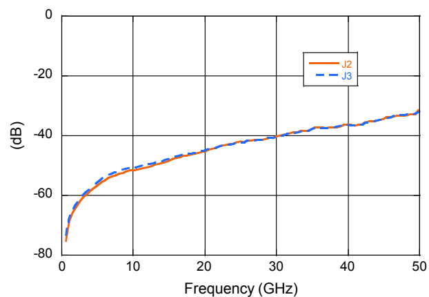
Isolation @ +10 mA
