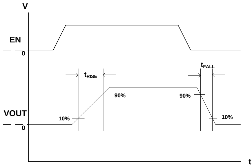
Figure 1. Output Rise/Fall Time
