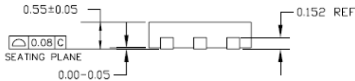
SIDE VIEW
