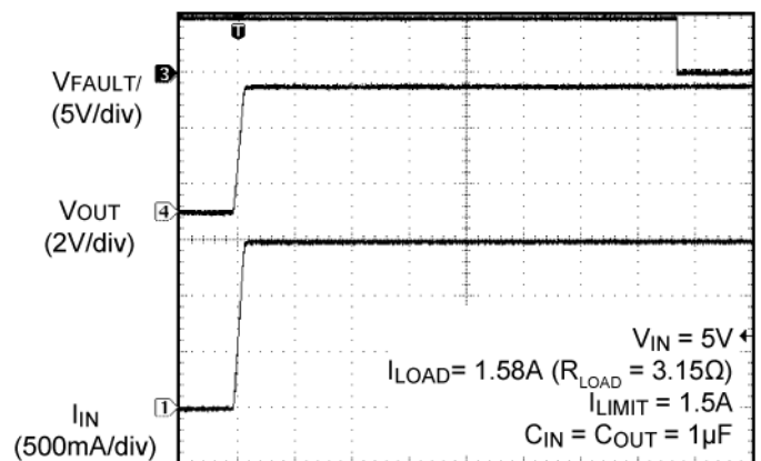
Turn-On Into Minimal Overload - 1.5A I_{LIMIT}
