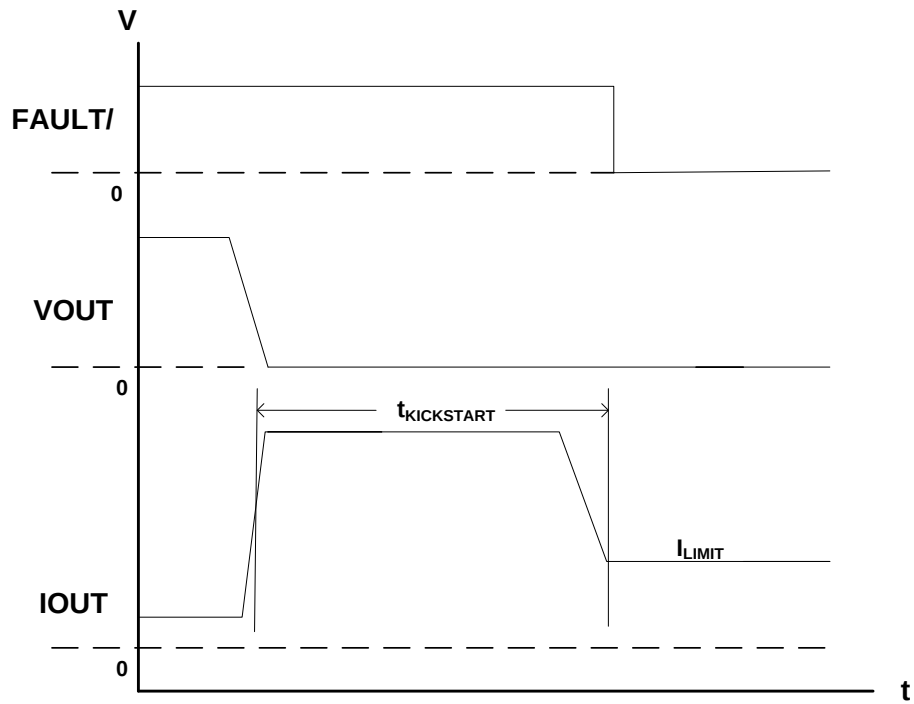
Figure 4. Overcurrent Fault Flag Delay (Kickstart)
