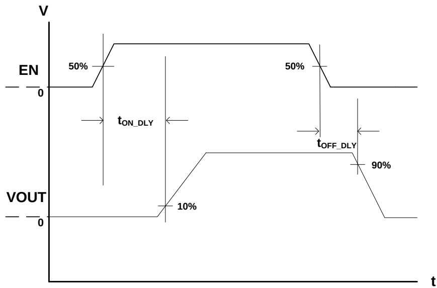
Figure 2. Turn-On/Off Delay
