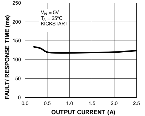
FAULT/ Response Time vs. Output Current
