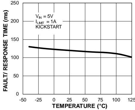
FAULT/ Response Time vs. Temperature
