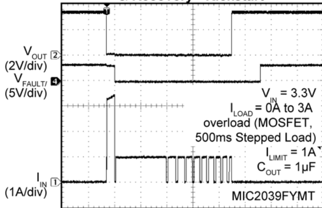
Time (100ms/div)
