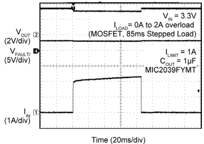
Output Thermal Shutdown & Recovery
