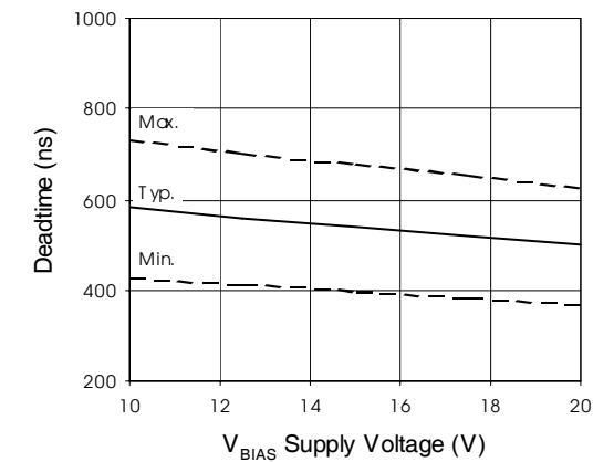
Figure 11B. Deadtime vs. Supply Voltage
