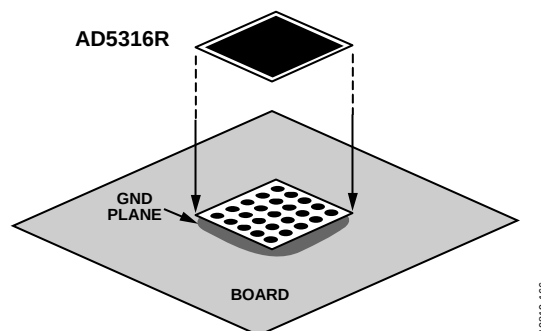
Figure 51. Paddle Connection to Board
