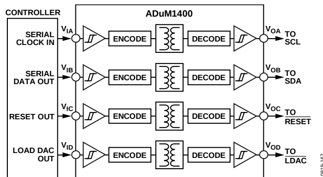
Figure 52. Isolated Interface
