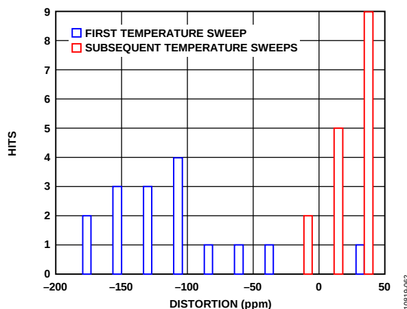
Figure 49. Thermal Hysteresis
