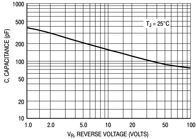
Figure 19. Typical Capacitance
